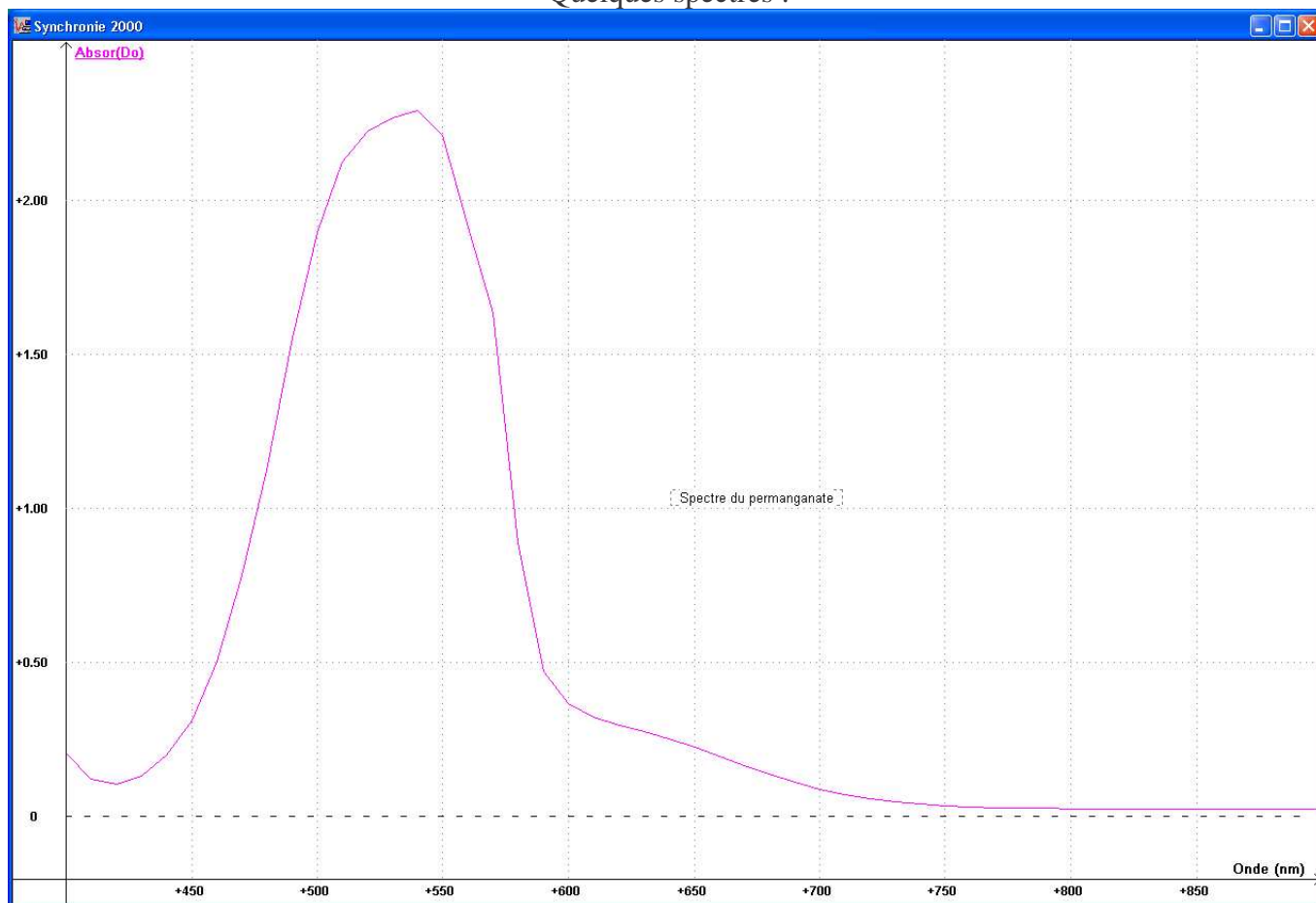
Spectre du permanganate
